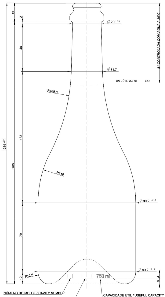
VISTA FRONTAL / FRONT VIEW
